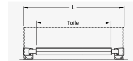
Guidage coulisses
