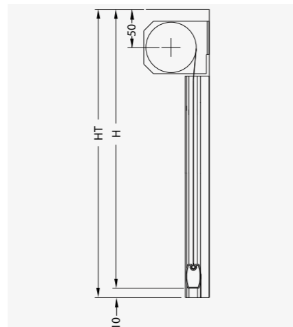
Guidage coulisses
