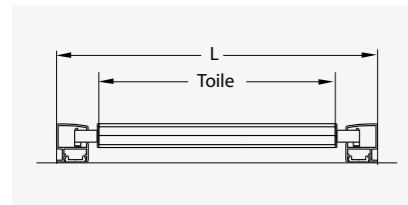
Guidage coulisses
