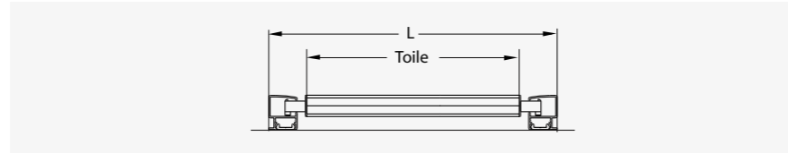
Guidage coulisses Fix
